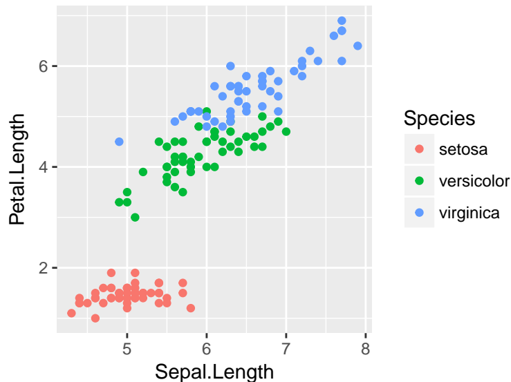
Figure 6: Iris Data
