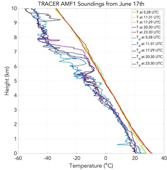
Figure A.1: June 17, 2022 TRACER AMF1 radiosonde soundings overlaid for the event day.
